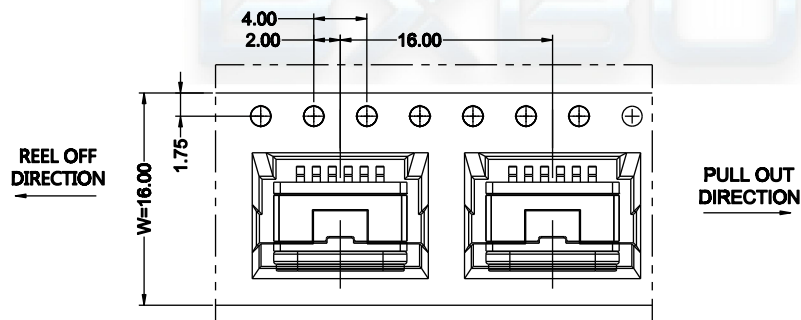
DETAIL X
