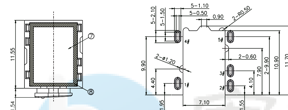
RECOMMENDED P.C.B. LAYOUT TOP VIEW (TOLRANCE:±0.05)
