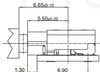
MATED CONDITION(REF.)
