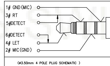
(ø3.50mm 4 POLE PLUG SCHEMATIC )
