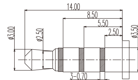
(3.5mm 4 POLE PLUG DETAIL DRAWING)
