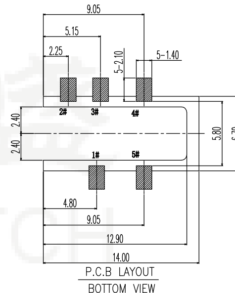
(Ø3.50mm 4 POLE PLUG )
