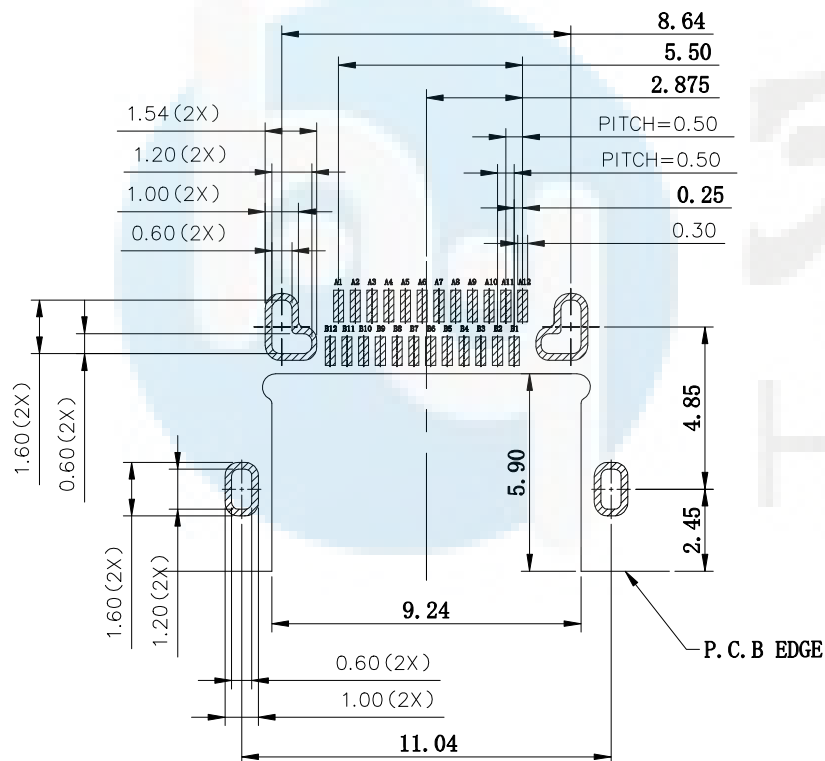
RECOMMENDED PCB LAYOUT(TOP VIEW)
