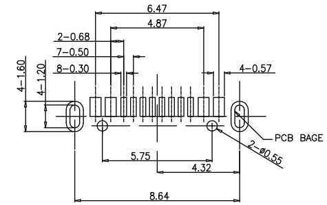
PCB LAYOUT GENERAL TOLERANCES: ±0.05
