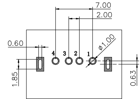
RECOMMENDED PCB LAYOUT (TOP VIEW) DEFAULT TOLERANCE+/-0.05 THICKNESS T=1.6mm
