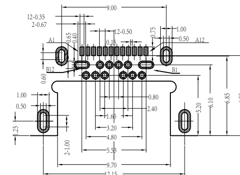
RECOMMEND PCB LAYOUT TOL= ±0.05 TABLE B
