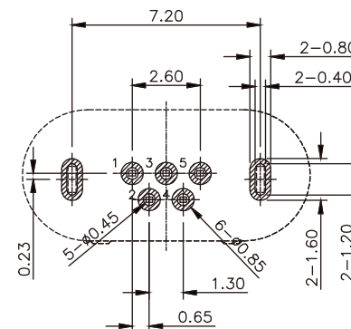
RECOMMENDED P.C.B. LAYOUT (TOP VIEW) GENERAL TOLERANCE: \pm 0.05
