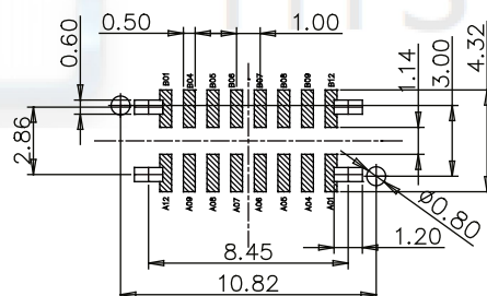
RECOMMENDED P.C.B. LAYOUT (俯视图) TOLERANCE UNSPECIFIED ±0.05mm
