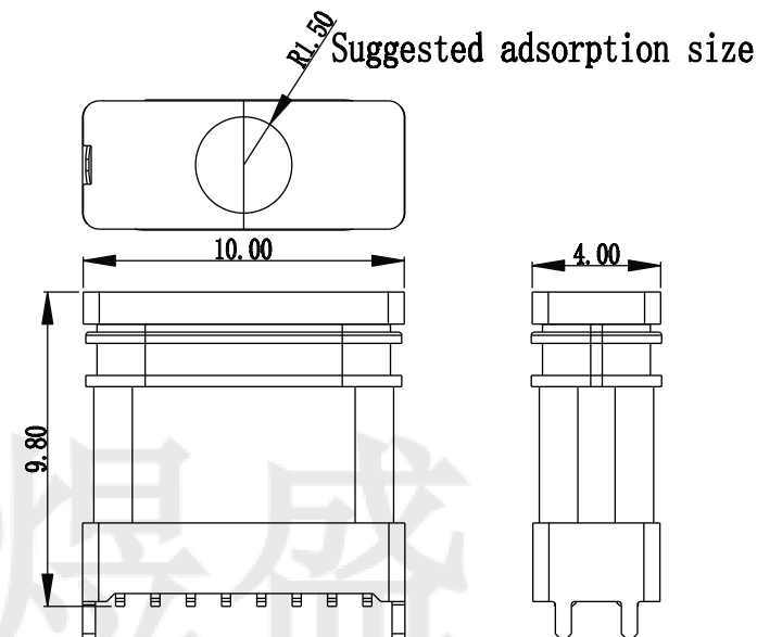
Install suction cap diagram
