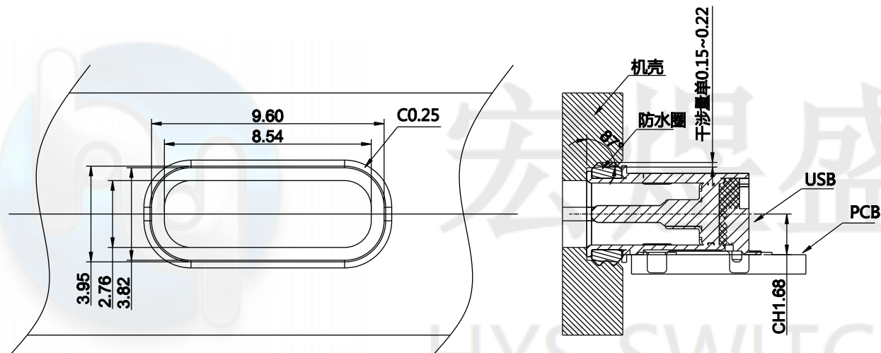
RECOMMENDED ASSEMBLY DRAWING
