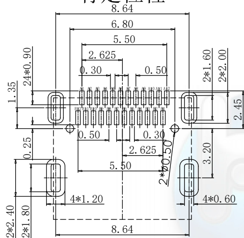
RECOMMENDED PCB LAYOUT, TOP VIEW (THICKNESS=1.0~1.2MM; TOLERANCE: \pm 0.05 )
