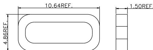
Suggested size of the waterproof ring
