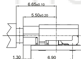
MATED CONDITION(REF.)
